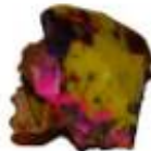
metamorphic
