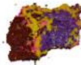
sedimentary
